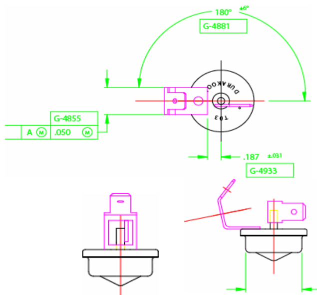
Drawing dimensions in inches.
